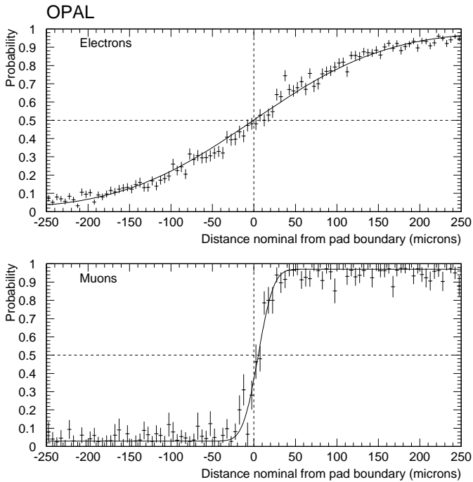
Fig. 13. The pad boundary images for test beam electrons and muons at layer 7. Each image is formed by plotting the probability that the pad with maximum signal lies above a given pad boundary as a function of the incident particle trajectory. The measured pad boundary bias is the difference between the intersection of the fitted curves for electrons and muons with the 0.5 probability level. The horizontal axis is in micro-strip coordinates only nominally centered on the pad boundary
