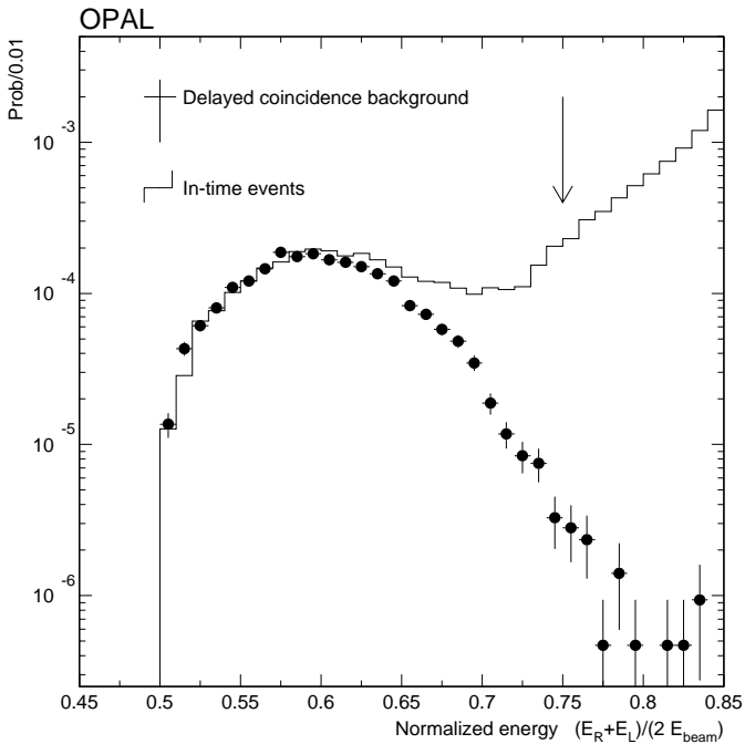
Fig. 24. The low energy tail of the total energy spectrum normalized to the number of accepted luminosity events for the 1994 data (histogram). The points with errors show the background spectrum derived from the delayed-coincidence triggers. The arrow indicates the position of the selection cut made on the average energy
