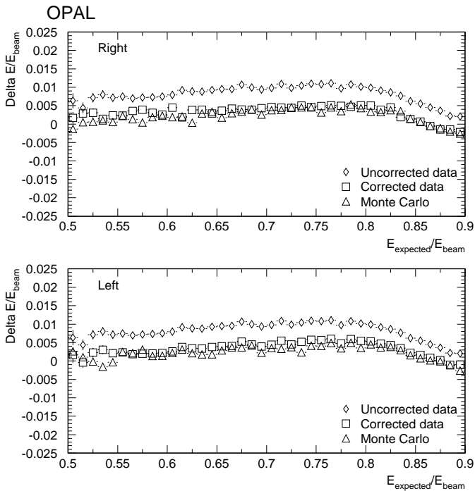
Fig. 22. Fractional difference between the expected energy (calculated from the radii of the scattered electron and positron) and both the corrected and uncorrected measured energy for the sample of acollinear events. Also shown is the difference expected from the detector simulation. The apparent nonlinearity visible in both the data and the Monte Carlo above a fractional energy of 0.8 arises from effects of the finite size of the LEP beams and their divergence convoluted with the rapidly falling spectrum of initial state radiation
