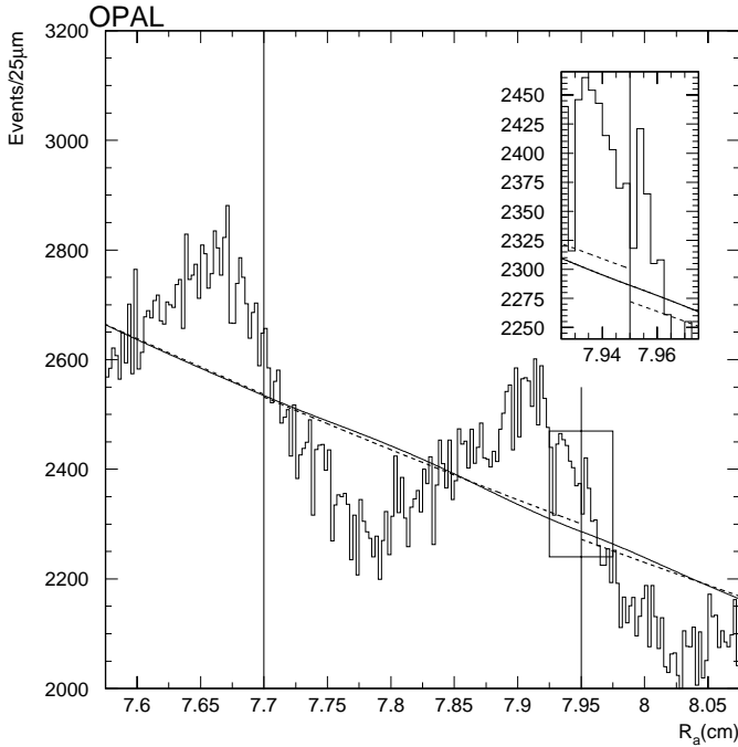
Fig. 11. The observed distribution of the raw radial coordinate, R_a , and the target function for dN/dR_{\text{smooth}} in the region near the inner acceptance boundary. The vertical lines indicate the position of the pad boundaries in the reference layer of the calorimeter. The departure of the pad by pad R_a distribution from R^{-3} causes the steps between the virtually straight power-law segments (dashed lines) given by the a_i . The final target function is indicated by the solid curve. The inset shows how the final target function passes smoothly through the mid-points of the power-law discontinuities at the pad boundaries
