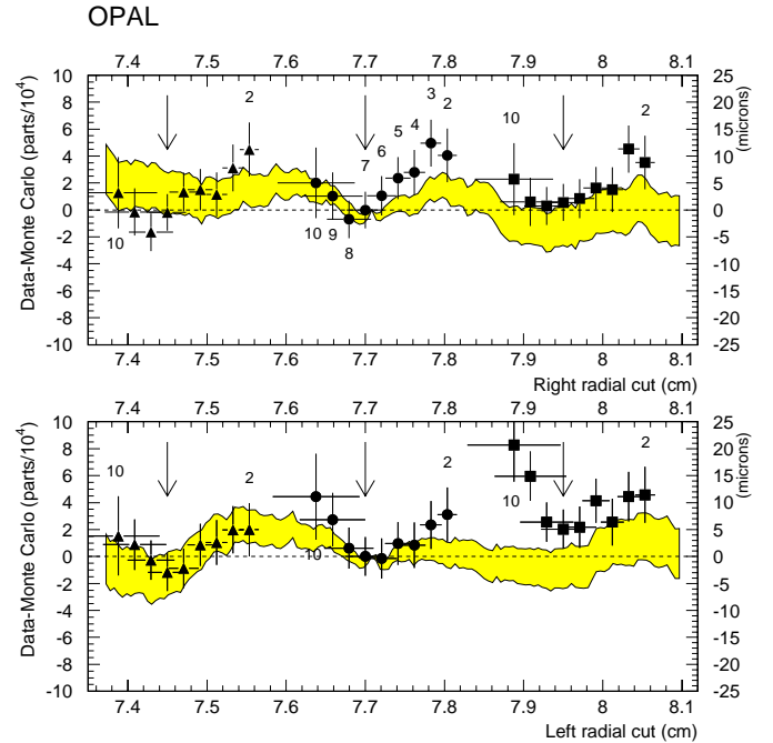
Fig. 17. The shaded band shows the relative change in acceptance between data and Monte Carlo as a function of the definition cut on the inner radius for the SWITR and SWITL selections for the combined 1993–1994 data sample. Departures from zero beyond the highly correlated one-sigma statistical errors which correspond to the width of the band are due to the small residual structure in the reconstructed radial coordinate. The solid points show the coordinate bias measured by the anchoring procedure. The primary anchor at 7.7 cm is fixed to lie at zero. The deviations of the other anchors from the data/Monte Carlo band show the acceptance shifts which would result if any of the alternative pad boundaries had been chosen as the reference. Triangles, circles and squares indicate the 5–6, 6–7 and 7–8 pad row boundaries respectively. The numbers indicate the layer depth in radiation lengths. The arrows show the location of the radial pad boundaries at the center of measurement ( 7 X_0 )
