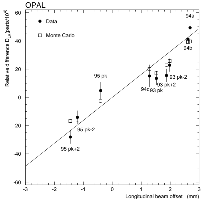
Fig. 29. D_{\text{LR}} , the difference between SWITL and SWITR selections, divided by their average, as a function of the mean measured longitudinal offset of the beam spot. The points show the value for each of the nine data taking periods for both the data, and the detector simulation. The detector simulation uses the reconstructed longitudinal beam position and the transverse offsets and tilts as inputs. The solid line shows the expected ratio if there were no effects from energy resolution and from differences in the eccentricities of beam in the left and right calorimeter
