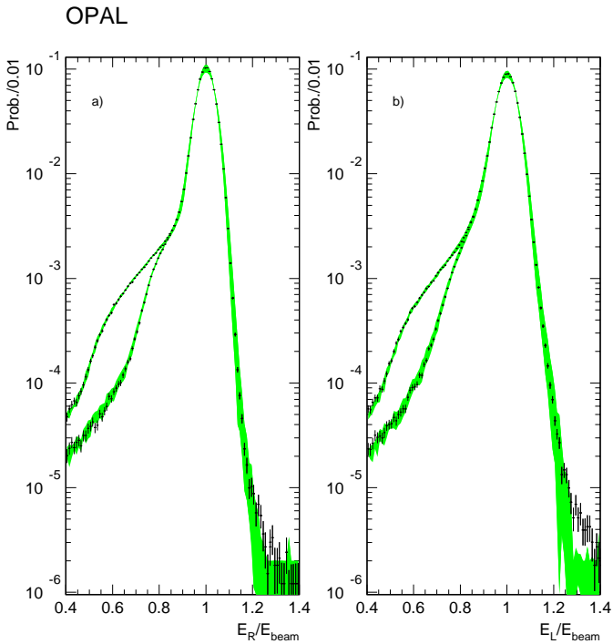
Fig. 31a,b. The normalized energy distributions in the right a and left b calorimeter for events passing all geometric cuts for the SWITA selection and which in addition have more than 0.85 of the beam energy in the opposite calorimeter. The energy spectrum is shown respectively before and after the acollinearity cut has been applied in the upper and lower branches of the curves. The points with errors show the data. The shaded bands show the Monte–Carlo predictions for the range of energy parameterizations used in assessing the systematic error (see Sect. 4.3). Above 0.8 the upper and lower branches of the curves are nearly indistinguishable
