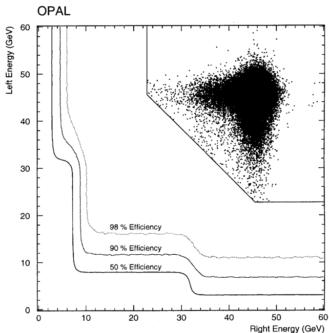
Fig. 26. Left versus right summed energy for 10^5 SWITA selected events in 1994 with calculated 50, 90, and 98 % efficiency contours for the combined SWSEG, SWHILO trigger signals for the threshold settings. The straight lines indicate the energy cuts imposed in selecting the SWITA sample
