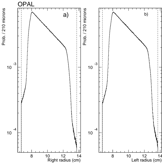
Fig. 35a,b. The distributions of R_R after all SWITL selection cuts have been applied a , and of R_L after all SWITL selection cuts have been applied, b . The points and error bars are the data and the histogram the Monte Carlo. The vertical dotted lines indicate the radial isolation cuts
