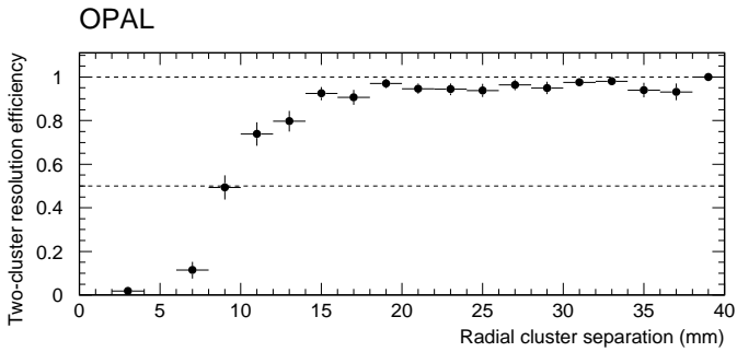
Fig. 7. The measured probability of reconstructing the second cluster in a radiative Bhabha event, where the second cluster energy lies between 5 and 10 GeV and it shares the same azimuth as the primary cluster, plotted as a function of the radial separation between the two clusters
