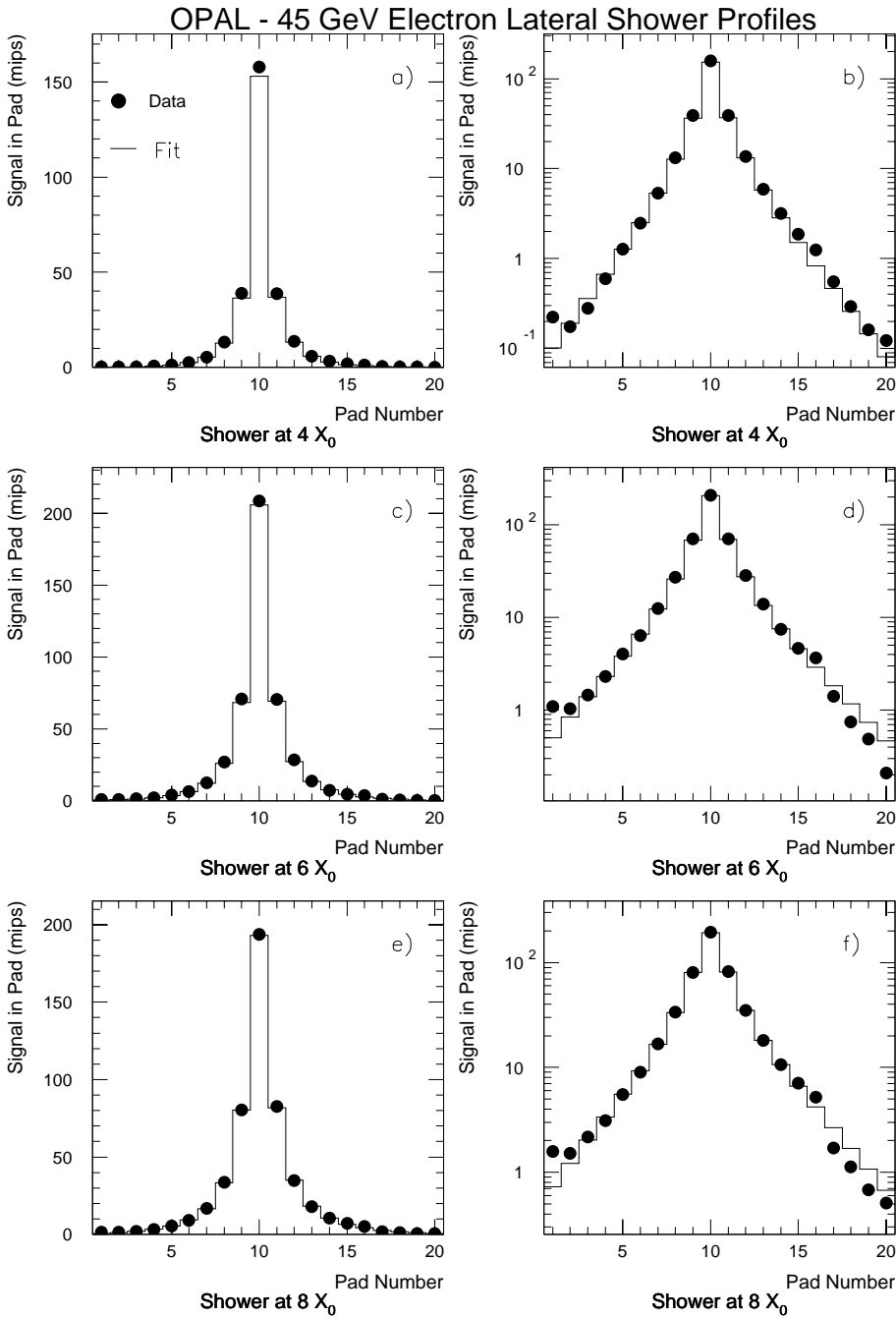
Fig. 6a–f. Average radial shower profiles at 4 X_0 a and b , 6 X_0 c and d , and 8 X_0 e and f . The fit shows the parameterization of the electromagnetic showers given in [17]. The left plots show the data on a linear scale, the right plots on a logarithmic scale
