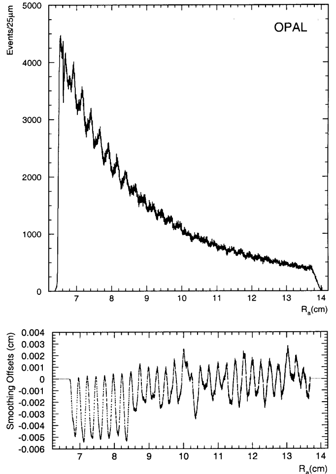
Fig. 10. The distribution (upper plot) of R_a , the raw radial coordinate, averaged over layers, for the largest of the 9 luminosity analysis data sets (94b). Also shown (lower plot) is the bin-by-bin smoothing offsets, S(R_a) , determined by the smoothing condition. The quasiperiodic structure at the 2.5 mm period determined by the pad width has a maximum amplitude of \approx 50 \mu\text{m} . The Bhabha isolation cuts have been applied, except for those involving the radial coordinate in either calorimeter
