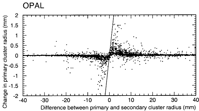
Fig. 8. The displacement of the radial coordinate of the highest energy reconstructed cluster in the “overlaid” radiative event sample, as a function of the radial separation between the primary and secondary clusters. Here the secondary cluster is selected to have an energy above 2 GeV. The diagonal line shows the expected displacement if the secondary cluster were simply mistaken for the primary
