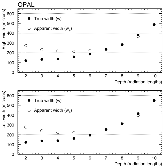
Fig. 15. Apparent and estimated true values of the pad-boundary transition width, w , at the boundary between pad rows 6 and 7 (7.7 cm). The upper plot shows the right side, the lower plot the left side. The errors on the estimated true width reflect the uncertainty in the conversion of w_a to w
