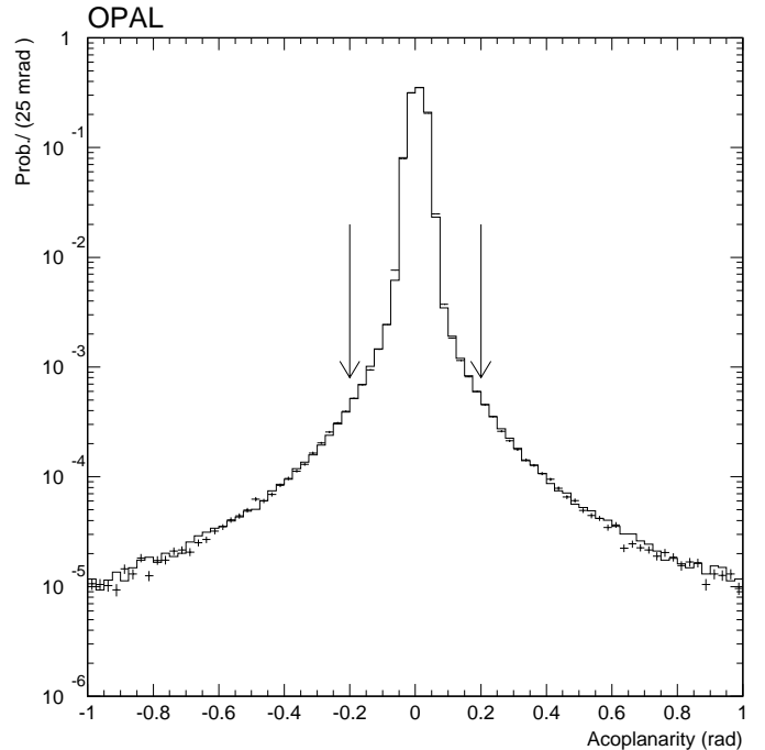
Fig. 34. The distribution of the acoplanarity ((\phi_R - \phi_L) - \pi) after all the SWITA selection cuts have been applied, except for the acoplanarity cut. Data are shown as points and Monte Carlo as the solid histogram. For this comparison, the background from accidental coincidences of off-momentum beam particles has been subtracted from the data. The acoplanarity cut is indicated by the two vertical arrows. The mean acoplanarity is offset from zero by 6.2 mrad averaged over all fills. This can be compared with the expected effect due to the OPAL magnetic field, which is 6.34 mrad
