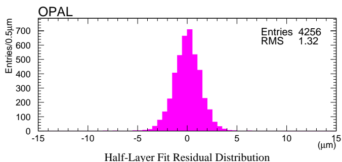
Fig. 4. The residuals of the individual detector radii from the fit half-circles for all the standard metrology measurements. The RMS of 1.32\mu\text{m} includes the relative precision achieved in placing the the individual detectors on each half-ring, as well as the resolution of the subsequent measurements of their positions
