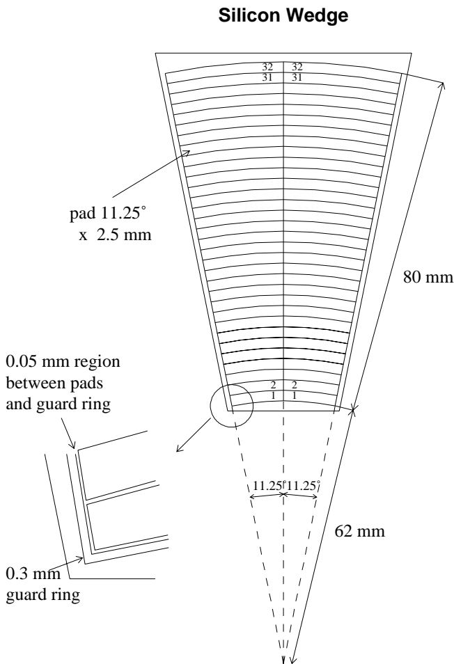
Fig. 2. A schematic illustration of the silicon diode pad geometry. The silicon detectors are divided into 2 rows of 32 pads, each covering 11.25^\circ in azimuth. The radial pad segmentation is 2.5 mm. Silicon detectors within each layer of the calorimeter are physically overlapped, so that the azimuthal boundaries of their active regions coincide and there are no dead or “double counted” regions
