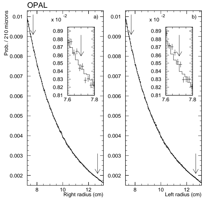
Fig. 36a,b. The distributions (after the isolation cuts have been applied) of R_R a , and R_L b . The arrows indicate the location of the definition cuts for the SWITR and SWITL selections. The points and error bars are the data and the histogram the Monte Carlo. The insets show fine details near the inner acceptance boundaries
