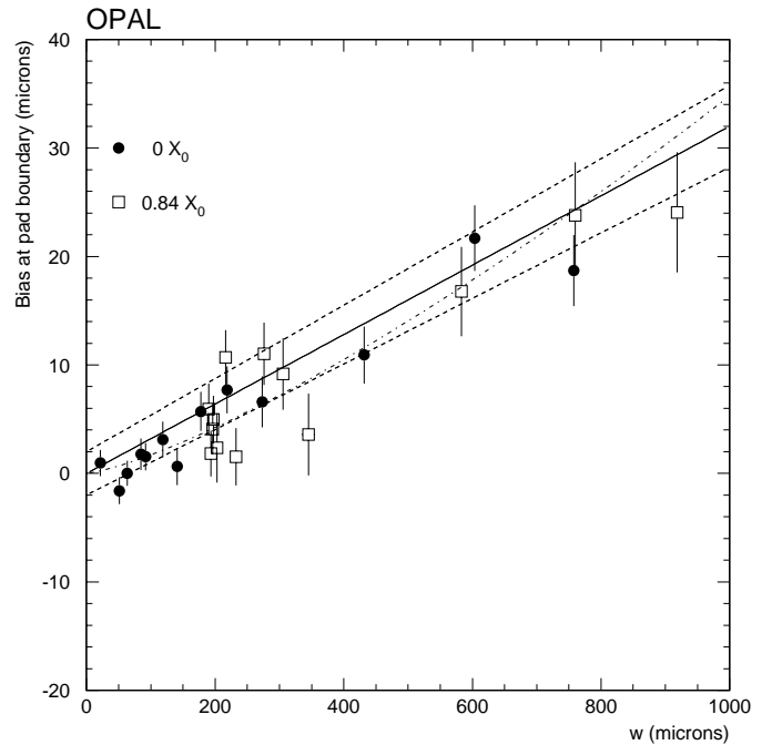
Fig. 14. The pad boundary bias as a function of the measured pad boundary transition width ( w ). The data points correspond to measurements at different depths in the calorimeter. The solid circles show the bias for the bare calorimeter ( 0 X_0 ) and the open boxes the calorimeter behind additional dead material ( 0.84 X_0 ). The line was fitted to the 0 X_0 data. The dotted lines show the error assigned to the parameterization. The dash-dotted lines shows an alternative two parameter fit of the form ax^b
