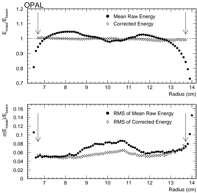
Fig. 20. Mean raw measured energy and its RMS for a sample of collinear Bhabha electrons (solid dots), as well as the mean corrected energy and its RMS for the same sample (open diamonds). All quantities are shown as a function of radius for the left calorimeter. The correction algorithm ensures that the energy response of the calorimeter is not a function of radius, and recovers almost all of the resolution lost to preshowering in the region between 9 and 11 cm, where the amount of upstream material exceeds 2X_0 . The vertical arrows indicate the position of the loose radial cuts. No clusters beyond these limits are used in the luminosity measurement
