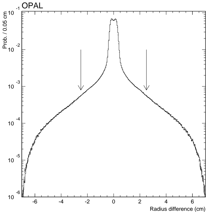
Fig. 32. The distribution of R_R - R_L after all the SWITA selection cuts have been applied, except for the acollinearity cut. Data are shown as the points and Monte Carlo as the solid histogram. For this comparison, the background from accidental coincidences of off-momentum beam particles has been subtracted from the data. The acollinearity cut is indicated by the two vertical arrows
