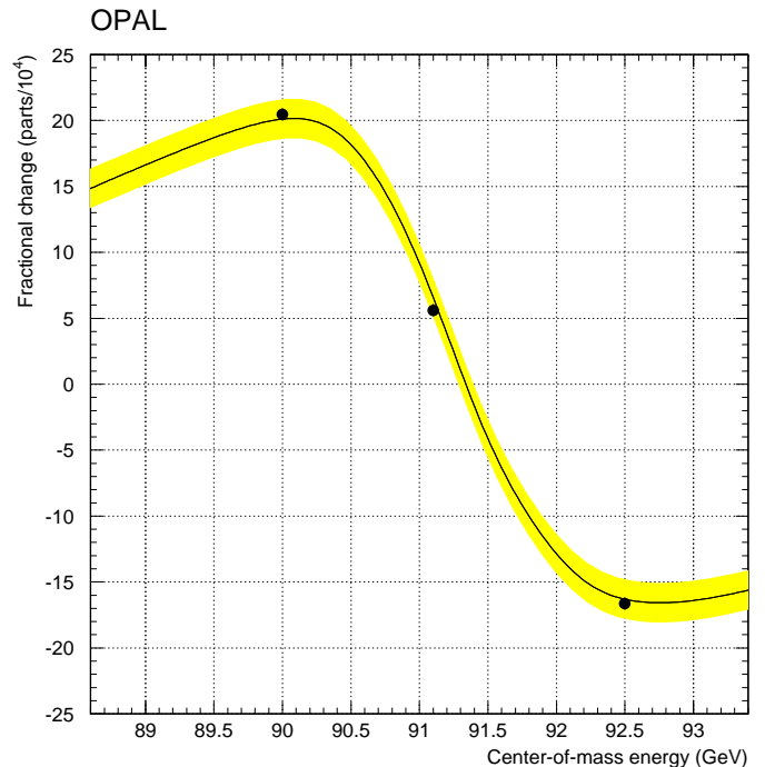
Fig. 30. Relative size of the energy dependence of the SiW acceptance as a function of center-of-mass energy near the Z^0 peak, excluding the fundamental 1/s dependence of the cross section. The curve includes the effects of Z - \gamma interference and the variation ( 6 \times 10^{-4} ) in vacuum polarization. The band gives the error assigned to this correction. The points with barely visible (statistical) error bars display the result of direct calculations at three energy points using BHLUMI 4.04
