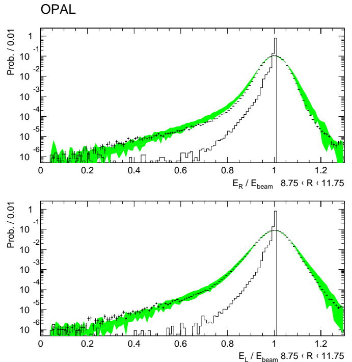
Fig. 21. The observed detector energy response to very collinear events, with |R_R - R_L| < 1 mm, (points) which is used to parameterize the detector simulation (shaded band) for showers in the radial region between 8.75 and 11.75 cm. The width of the shaded band shows the variation in the parametrization used in setting the systematic error. Because of the tight acollinearity cut applied to the samples, single radiative and double radiative events are highly suppressed, and the observed distribution is dominated by resolution effects, as illustrated by the narrow histogram of the bare BHLUMI four-vectors, whose tail falls two orders of magnitude below the simulated detector response
