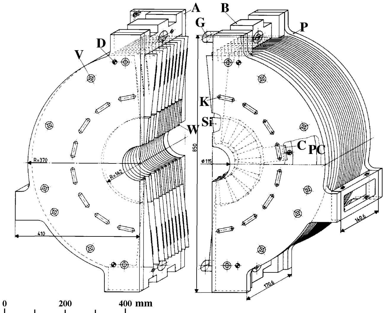
Fig. 1. An isometric view of one of the SiW calorimeters, separated into two C's, A and B. The 15 mm precision dowels which radially align the individual half layers are labeled as D. The holes for the cooling pipes are labelled as K. The clamps which fix the axial position of the half layers is also constrained by bolts and spacers at locations V, as well as by spacers at the inner bore. One of the brass dowels which align the two C's is labelled as G. On the left C, the beveled edges of the tungsten layers are visible and labeled as W. The silicon diode wedge structure in two successive layers is shown on the right C and labelled Si. Also shown on the right C is a PC motherboard (PC) and the ceramic hybrid (C). The dimensions shown on the figure are mm
