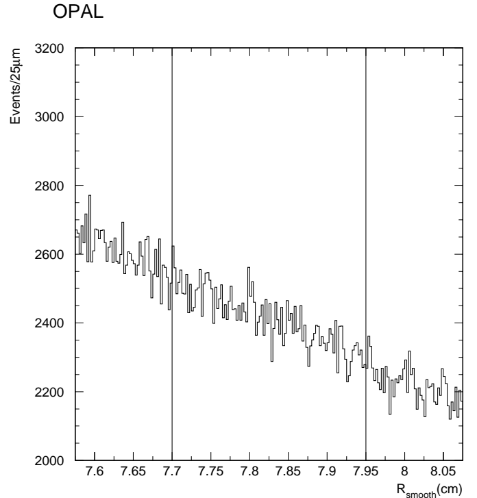
Fig. 12. The distribution of the smoothed radial coordinates near the inner cut boundary in the right side calorimeter for the 94b luminosity data sample, with all Bhabha isolation cuts applied, except for any cut at all on the radial coordinate in either calorimeter. The vertical lines indicate the position of the pad boundaries in the reference layer of the calorimeter. No structure is apparent beyond statistical fluctuations, and the measured luminosity is independent of the radius chosen to define the inner edge of the acceptance
