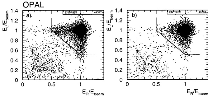
Fig. 18. The distribution of E_L vs E_R , after all the SWITA selection cuts have been applied, except for the energy cuts and the acollinearity cut a . The effect of the acollinearity cut on the radiative events and background is clearly visible in b . The lines in the E_L vs E_R plane indicate the cuts applied to the energies. The data shown here are from a typical run with approximately 40,000 SWITA events
