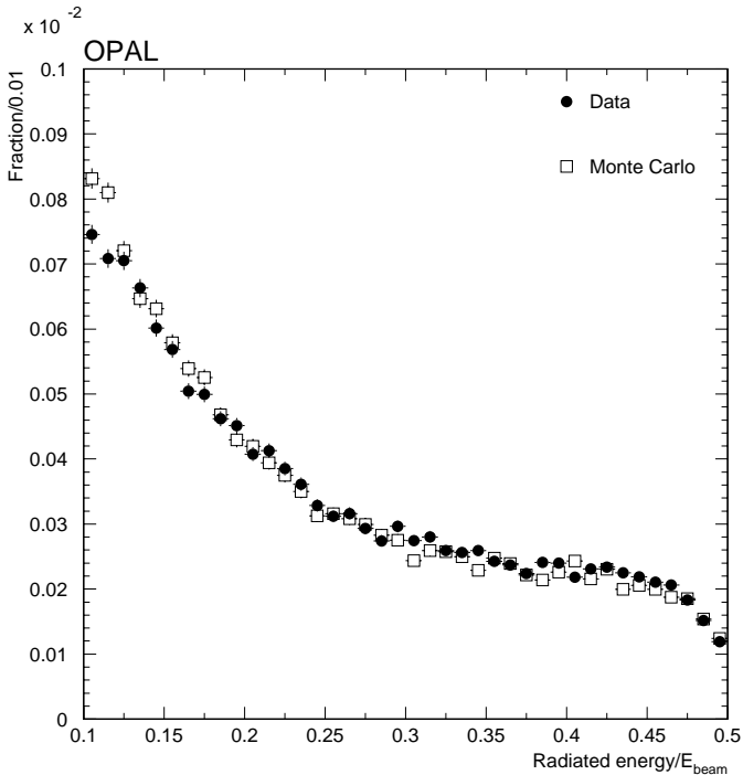
Fig. 33. The energy distribution of the least energetic cluster in SWITA events where the kinematic cluster selection algorithm has selected exactly one cluster on one side of the detector, and two on the other. To ensure a sample of kinematically complete events, we furthermore require that the total measured energy in the event is within 10% of the LEP center-of-mass energy. Only those clusters separated by at least 2 cm in radius or 400 mrad in azimuth are shown. Data and Monte Carlo are independently normalized to the total number of Bhabha events with a single full-energy cluster on one side of the detector
