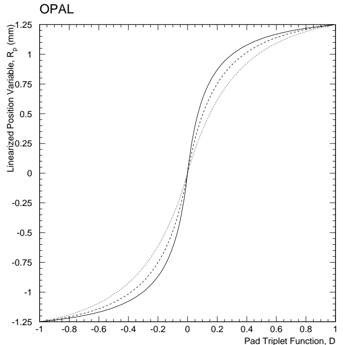
Fig. 9. The linearized position variable, R_p , in millimeters as a function of D , in units of half pad widths. This is shown for characteristic shower depths of 4 (solid line), 6 (dashed line) and 8 X_0 (dotted line). The center of the pad is at 0, and the boundaries at \pm 1.25\text{ mm}
