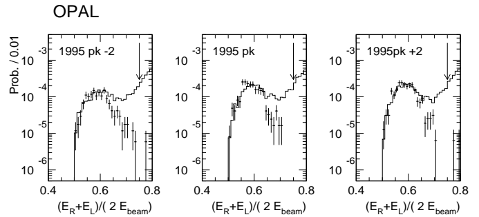
Fig. 25. The low energy tail of the total energy spectrum normalized to the number of accepted luminosity events for the three 1995 energy points. The data points show the accidental background as derived from the delayed coincidence accidental triggers and rescaled to account for the background distribution among bunchlets. The arrows indicate the position of the selection cut made on the average energy
