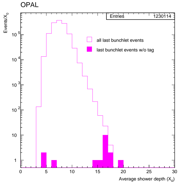
Fig. 27. The efficiency of the SiW wagon tagger as measured on the last bunchlet, where hold is always issued, independent of any tag. For the sample of accepted Bhabha events held on the last bunchlet, the average shower depth parameter is plotted for all showers (open) and showers lacking a tag (shaded). Showers with anomalous development profiles, either deeper or shallower than the wagon tagger layers, are seen to be the dominant cause of tagger inefficiency
