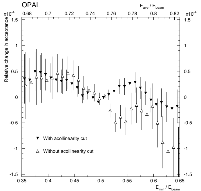
Fig. 23. The relative change in acceptance between the Monte Carlo and the 1993–1994 data as a function of scaling the energy cut. The observed deviations are well within the systematic error assigned to detector energy response. The error bars show the binomial uncertainties with respect to the standard cut values
