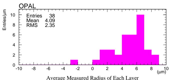
Fig. 5. The distribution of the average measured radii for each layer with respect to R_{\text{micro}} . The RMS of 2.4\mu\text{m} is due mostly to actual differences in the layer radii, since the error on each entry is typically less than 1\mu\text{m} . The abscissa is in units of \mu\text{m} relative to the microscope graticule
