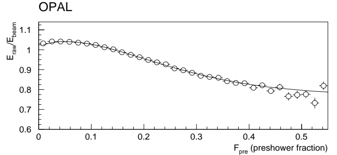
Fig. 19. Mean raw energy, E_{\text{raw}} , measured in the calorimeter as a function of the preshower fraction F_{\text{pre}} , for showers near the center of the acceptance in the left calorimeter. The solid line shows the functional form used for the energy correction
