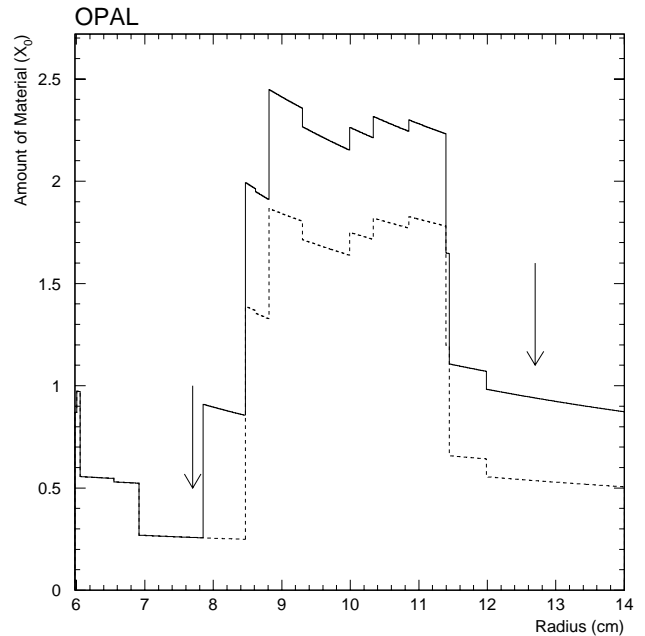
Fig. 3. The calculated material traversed by particles originating at the interaction point as a function of calorimeter radius, measured at the reference plane (246 cm) for the 1993–1994 detector configuration. The solid curve corresponds to the left, the dotted curve to the right side. The larger amount of material on the left is due to the passage of cables from the OPAL microvertex detector. The arrows show the location of the acceptance definition cuts on shower radius
