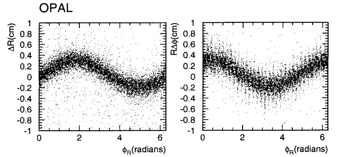
Fig. 28. The beam spot position can be determined with great precision from the measured coordinates of back-to-back Bhabha clusters. The plot on the left shows the acollinearity of non-radiative Bhabhas in the detector frame as a function of \phi_R . The plot on the right shows R times acoplanarity for the same sample
