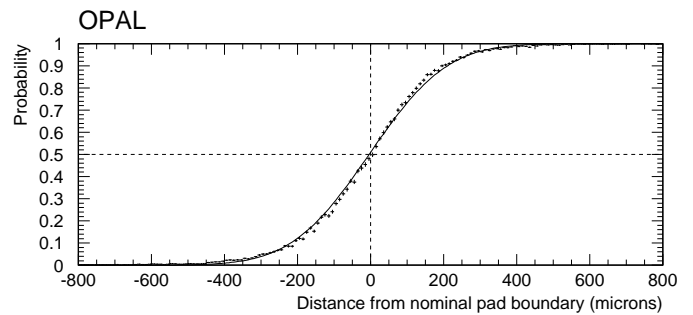
Fig. 16. The pad boundary image at LEP. The fraction of events with maximum in pad row 6 or beyond, as a function of distance from the pad boundary between rows 5 and 6, for the layer located after 7X_0 . The solid curve shows the fitted function
